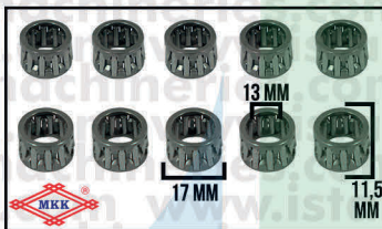
A43 BEARING PIN CRANK CS5200/5800
