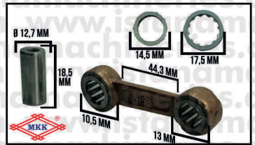
A42 CONROD KIT CS5800
