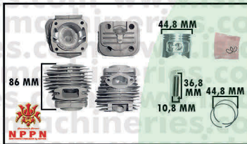
A1 CYL W/PISTON CS5200
