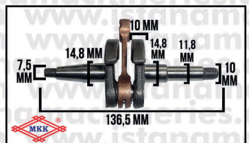
A39 CRANKSHAFT ASSY CS5200
