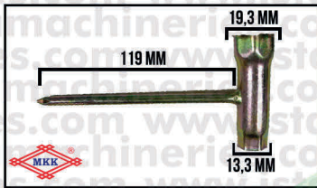
G6 KUNCI BUSI 13X19 "TBL+" CS5200/5800/658N
