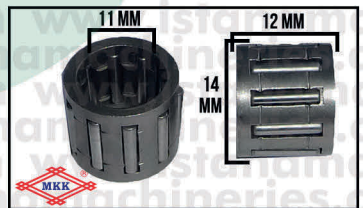
A37 BEARING PIN PISTON CS5200/5800
