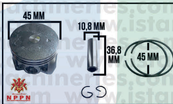
A33/36 PISTON ASSY CS658N
