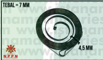
B29 REWIND SPRING "TIPIS" CS5200
