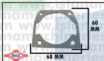
A10 GASKET CYLINDER BLOCK CS5200/5800
