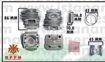
A1 CYL W/ PISTON (ULTIMATE) CS658N
