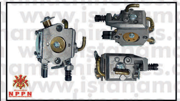
H1 CARBURATOR ASSY CS5200/5800
