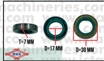
A-13 OIL SEAL CRANKSHAFT "BESI"
