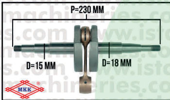
A-15 CRANKSHAFT
