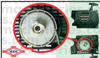
B25 RECOIL STARTER " 4K/2 PIR MD KOTAK" CS5800
