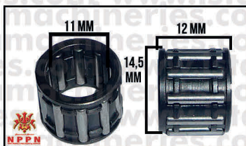
A37 BEARING PIN PISTON CS5200/5800
