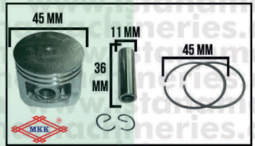
A33/36 PISTON ASSY CS5800
