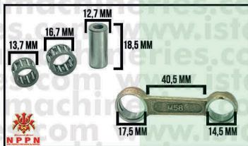
A42 CONROD KIT CS5200
