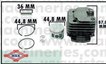
A1 CYL W/PISTON "HITAM" CS5200
