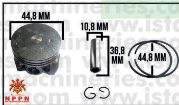
A33/36 PISTON ASSY CS5200
