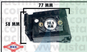
A6 CARBURATOR BRACKET FC5200/5800
