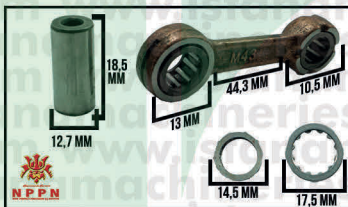
A42 CONROD KIT CS5800
