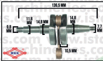
A39 CRANKSHAFT ASSY CS5800
