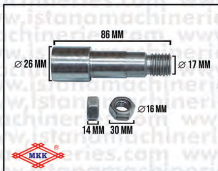
INTERMEDIATE GEAR SHORT SHAFT LM24A
