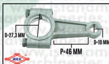
CONROD SCM 30
