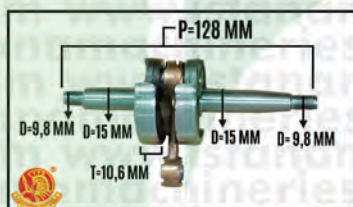
CRANKSHAFT 3WF-3
