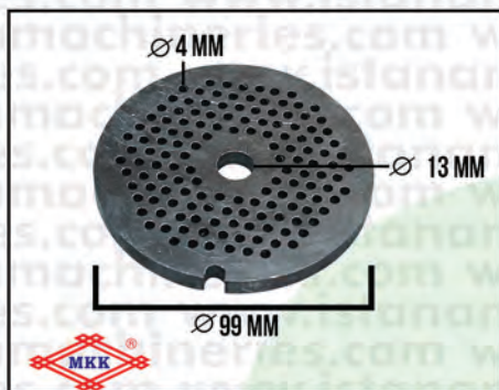
SARANGAN/PISAU GILANGAN DAGING 32 INCH 4MM
