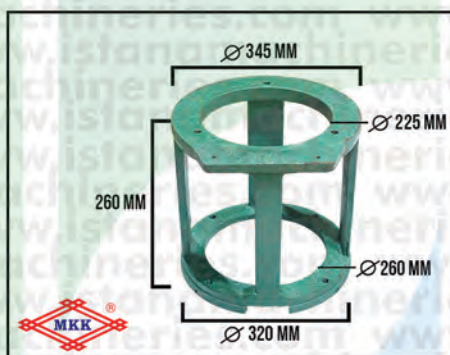
OUTER FRAME N120
