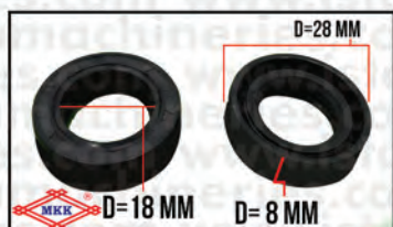
OIL SEAL 18 X 28 X 8 3WZ4/TU26
