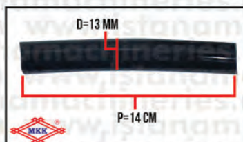
OVERFLOW HOSE 13MM *14CM 3WZ4/TU26
