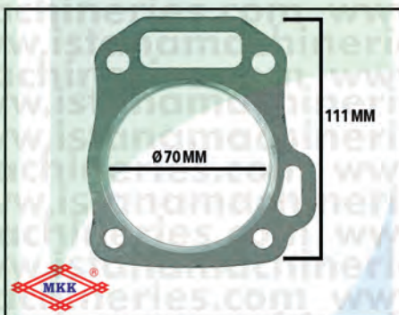
GASKET HEAD "PLAT" GX200
