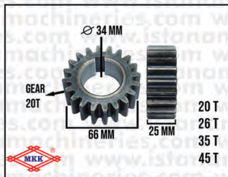
GEAR LM24A
