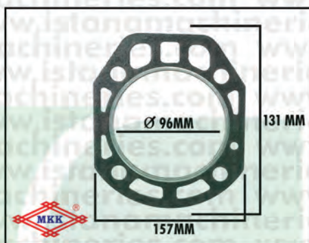
GASKET HEAD CF185
