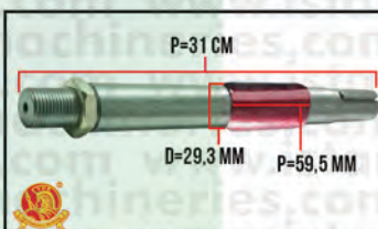
AS WATER PUMP NS80/3"
