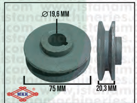
PULLEY SB10D
