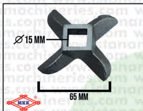
PISAU GILINGAN DAGING 32 INCH "MDL SILANG"
