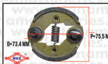
CLUTCH SHOE WHOLE SET 867/869
