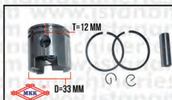
PISTON ASSY W/RING 33MM 3WZ4/TU26
