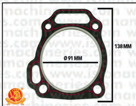
GASKET HEAD "SILICON" GX420
