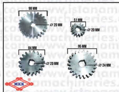
GEAR SET "GILINGAN TEBU" GZ-4
