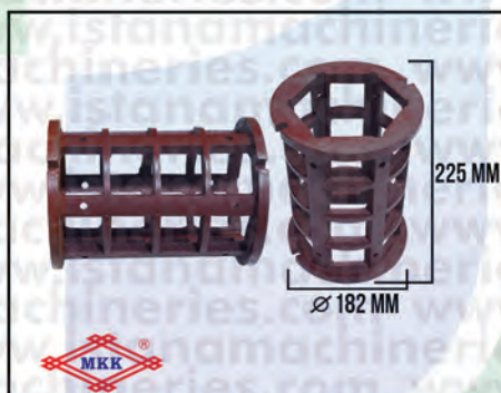
INNER FRAME N70
