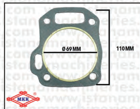
GASKET HEAD "KLINGRIT" GX160
