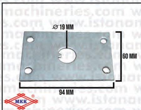
RING PLATE SB10D
