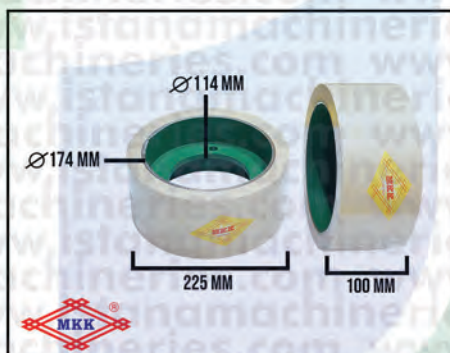
RUBBER ROLL 4 INCH
