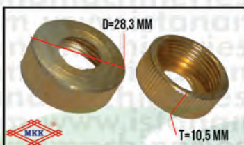
ADJUSTING NUT 3WZ4 / TU26
