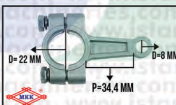
CONROD SCM 22
