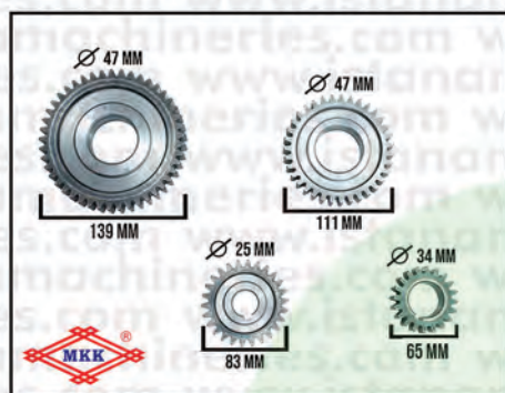
GEAR SET LM24A
