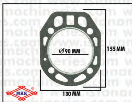
GASKET HEAD 2MM R180-QC/SW
