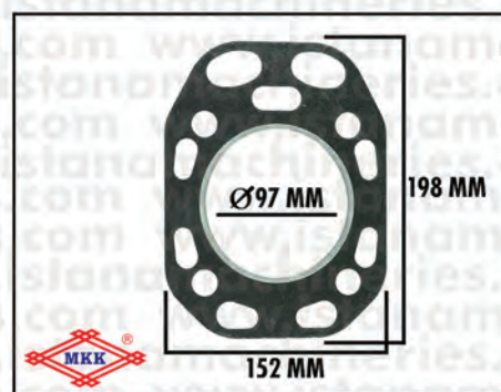
GASKET HEAD 2MM S195
