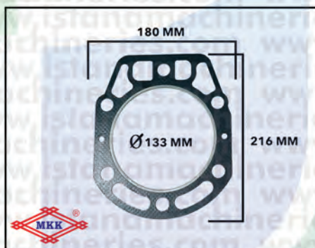
GASKET HEAD 2MM ZH1125
