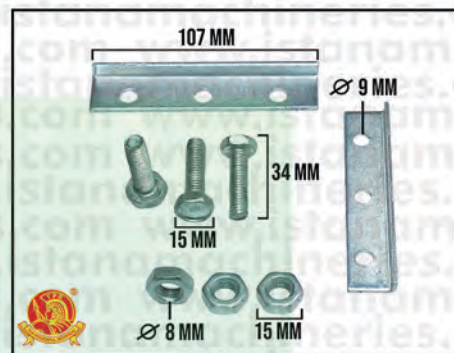
KLEM JACKSON BESI 4 INCH L-TYPE 3HOLE
