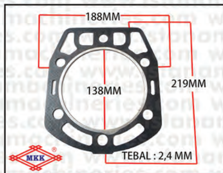
GASKET HEAD ZH1130/1133
