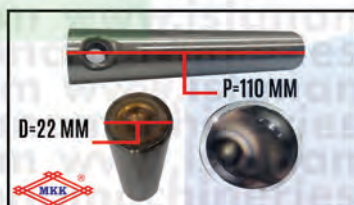
PLUNGER SCM 22
