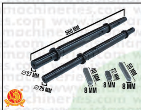
SHAFT "LONG" DRAT MODEL LM24A
