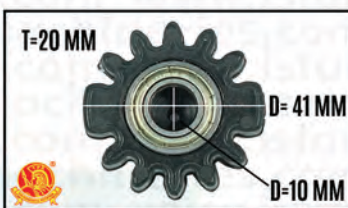
PLASTIC GEAR W/ BEARING SP/SFP 12
