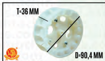
SEED ROLLER "BIG" SP/SFP-12
