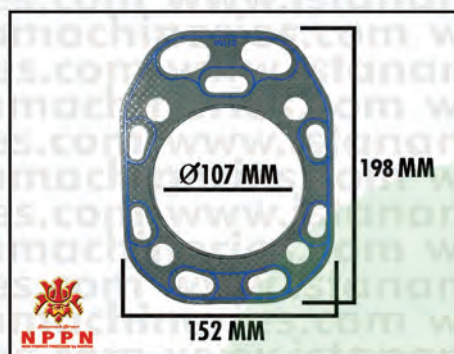
GASKET HEAD S1100-4H
