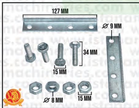
KLEM JACKSON BESI 5 INCH L-TYPE 4HOLE
