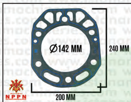
GASKET HEAD JD300
