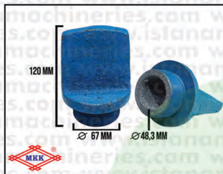
TUBE PLUG/TUTUP MAIN SHAFT "LONG" N120
