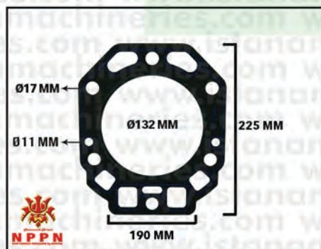
GASKET HEAD "ULTIMATE" S1125A
