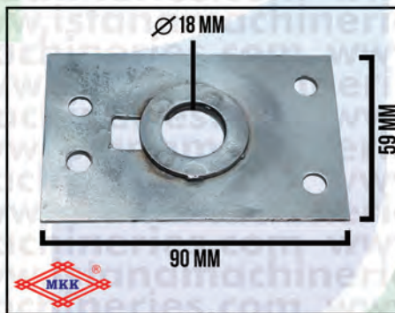
PLATE 211 SB10D
