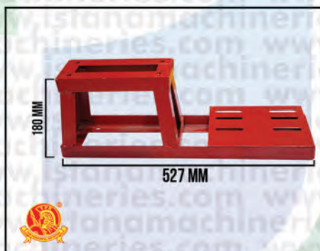
FRAME FOR DISK MILL FFC15
