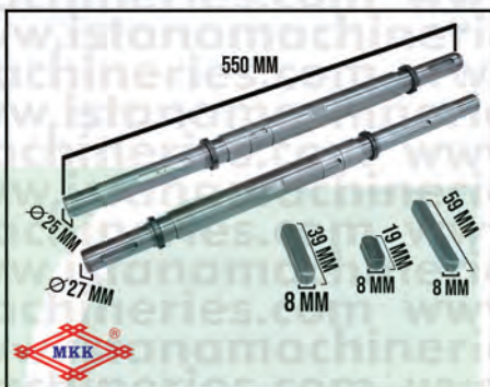
SHAFT "LONG" NUT/DRAT MODEL LM24A
