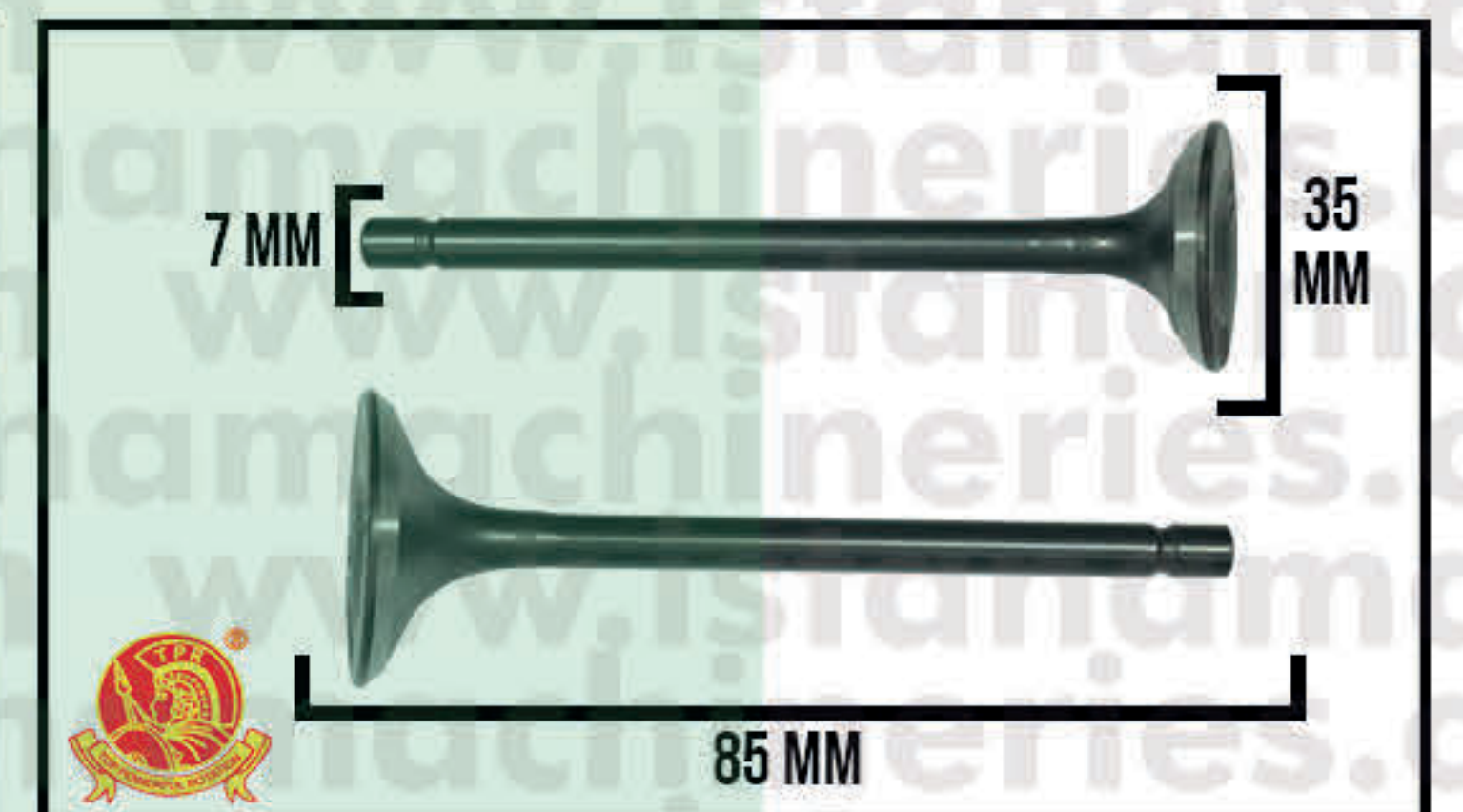
VALVE IN+EX "NEW" GX420>460
