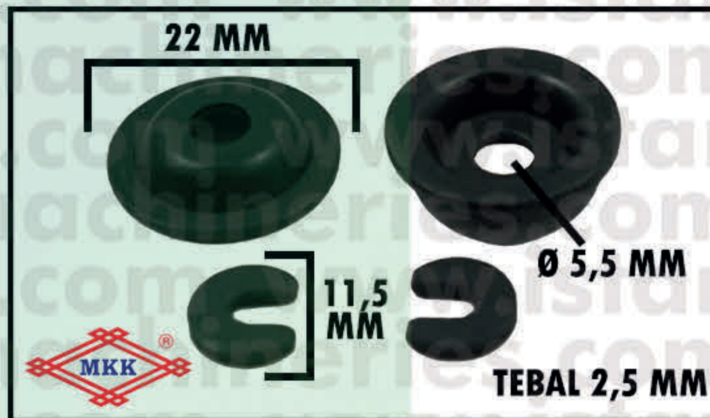
RETAINER MZ175
