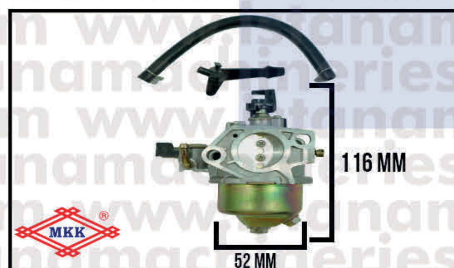
CARBURATOR "27MM" GX340>420
