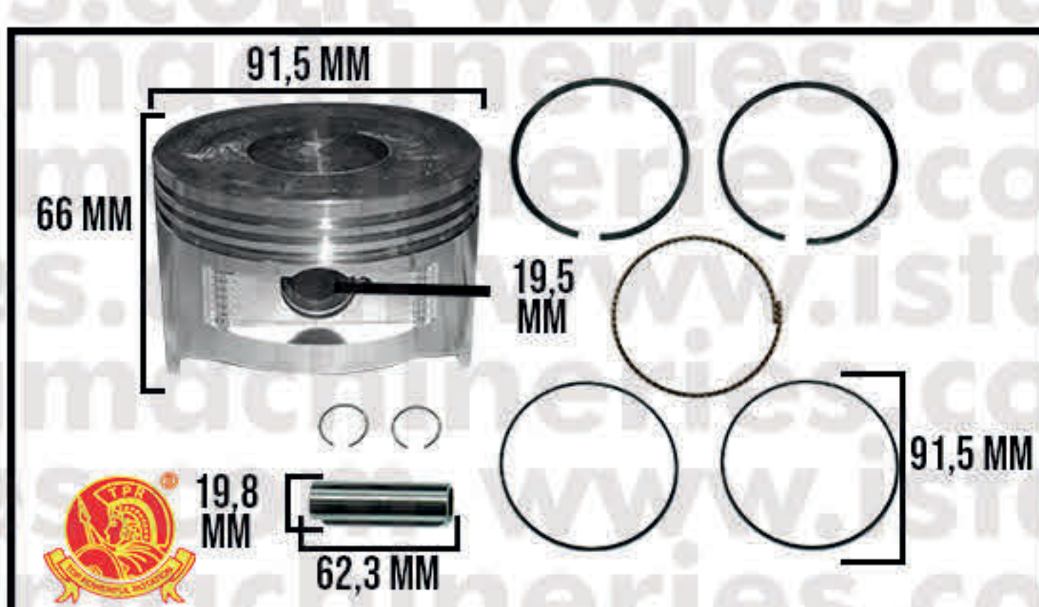
PISTON ASSY STD ET10000
