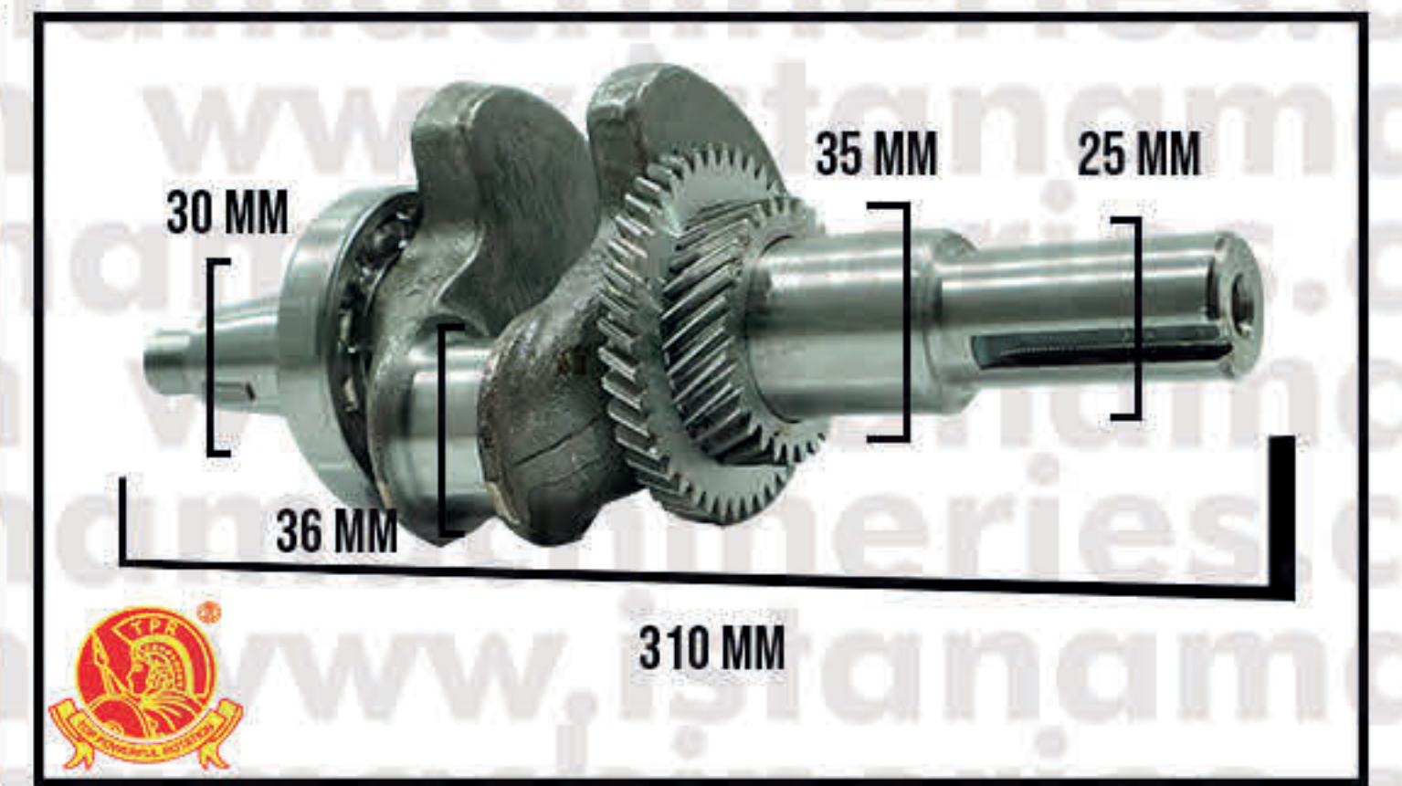
CRANKSHAFT SPIE "FOR ENGINE" GX390
