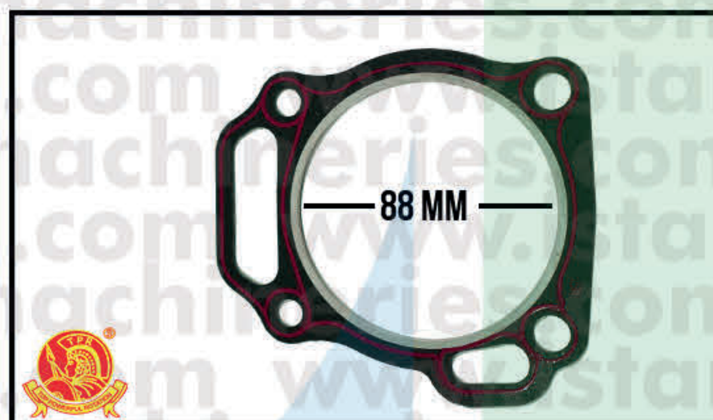
GASKET HEAD SILICON GX390
