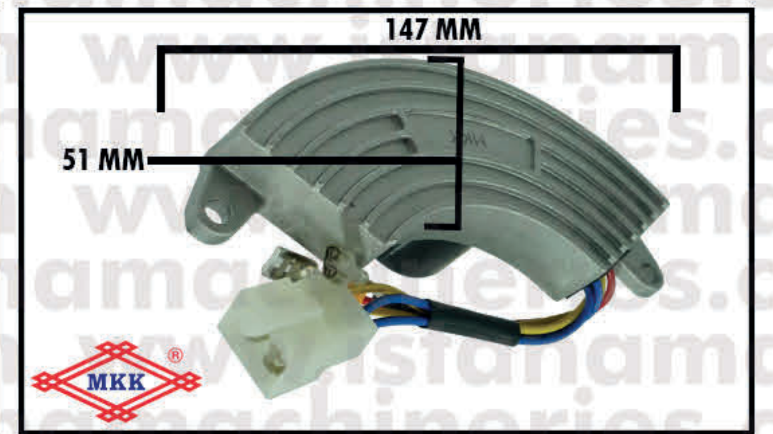
AVR ALUMINIUM-SABIT GFH6500
