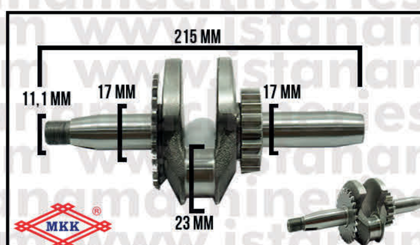
CRANKSHAFT ASSY "LURUS" ET1500
