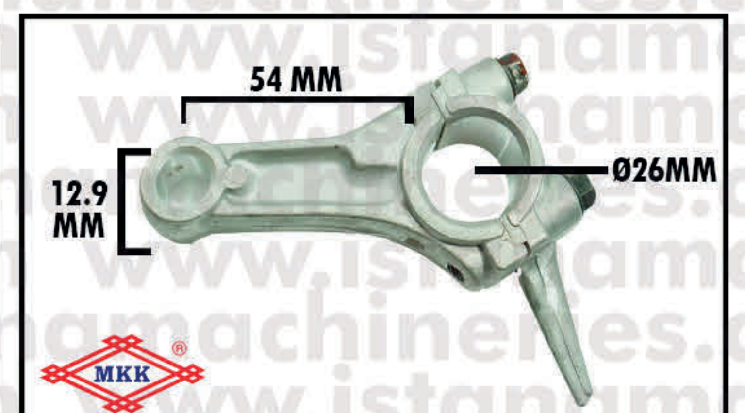
CONROD STD GX110>120
