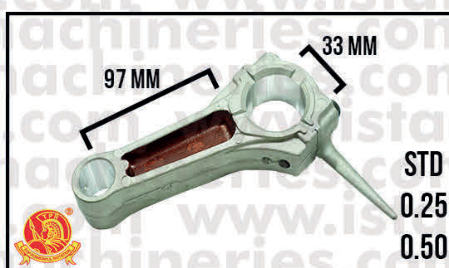
CONROD GX240/270
