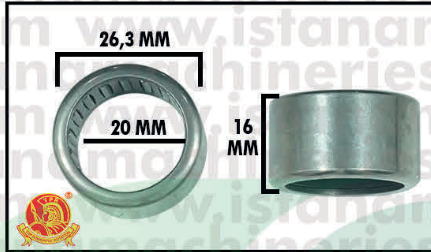
BEARING FOR GEAR REDUCTION BIG GX-200/220 "1/2 REDUCTION"
