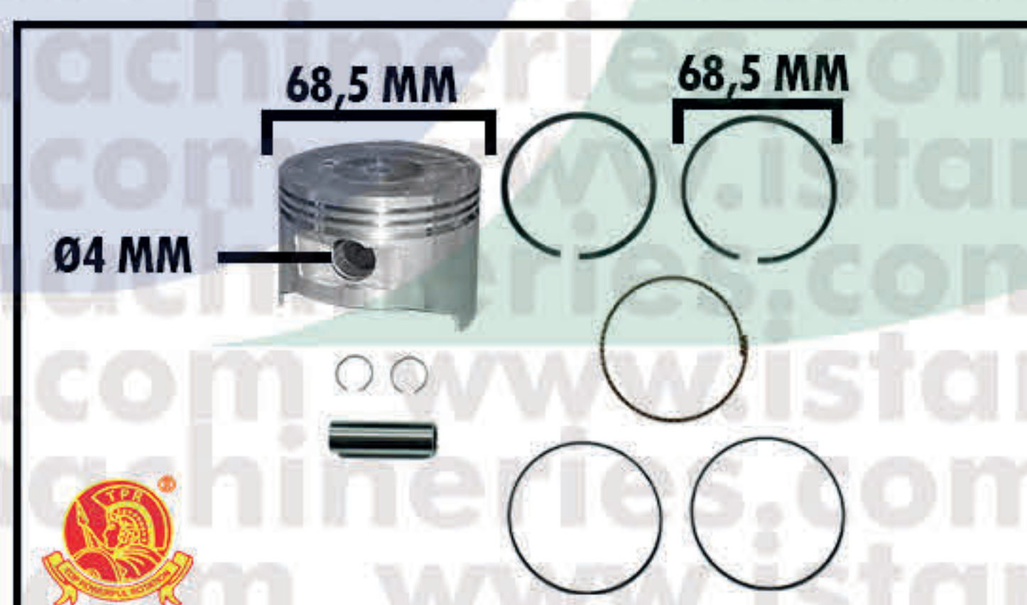
PISTON ASSY 0.50 GX200
