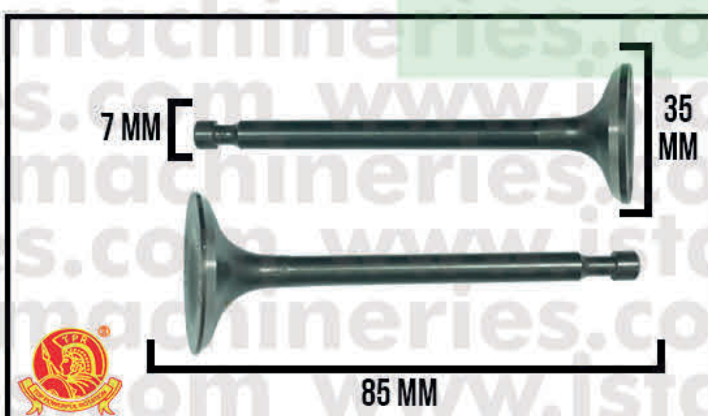
VALVE IN+EX "OLD" GX390
