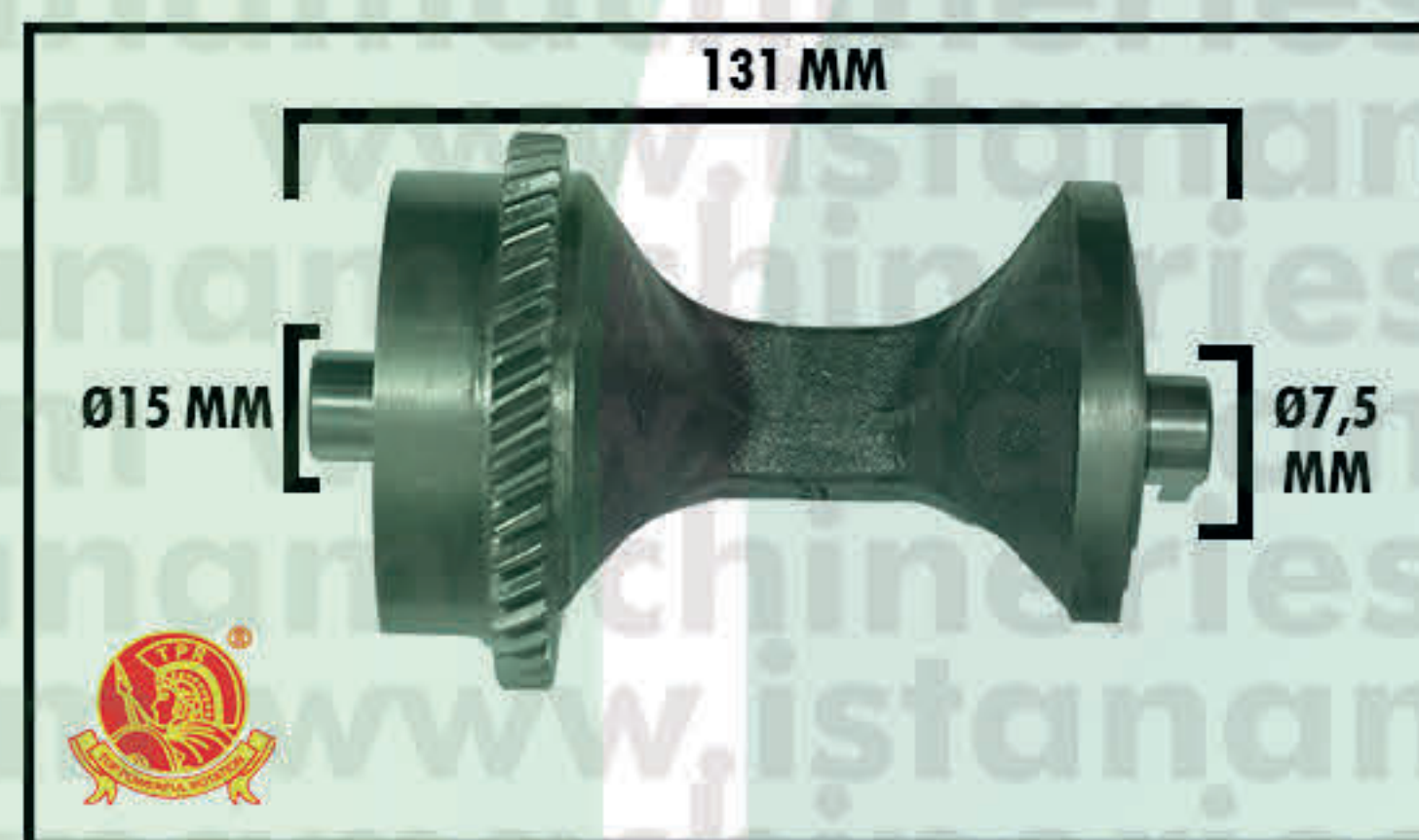
BALANCER SHAFT GX460
