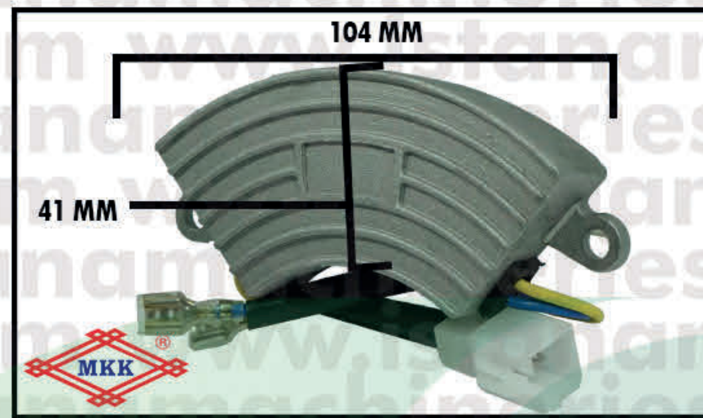
AVR ALUMINIUM-SABIT ET1500/GFH2500
