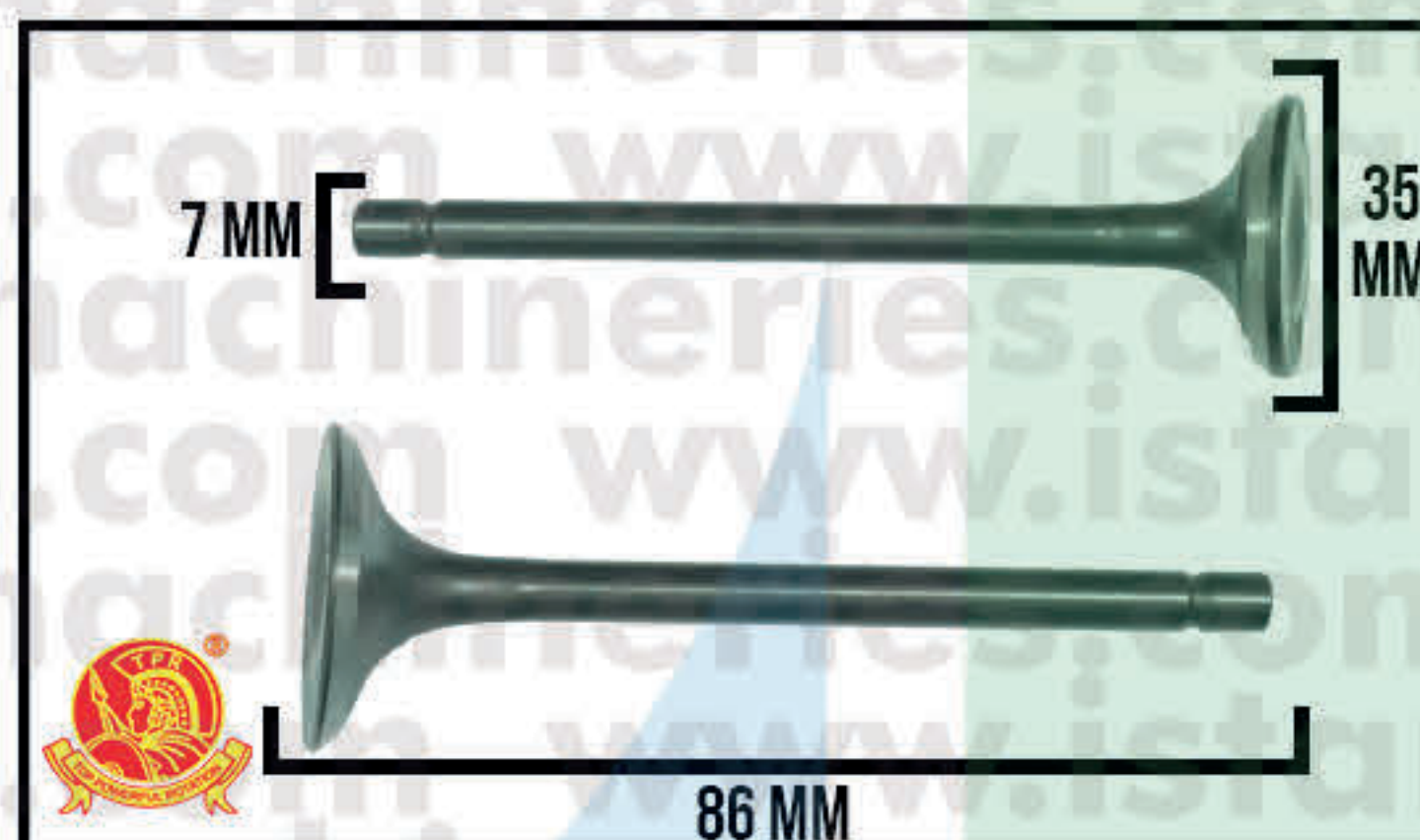
VALVE IN+EX "NEW" GX390
