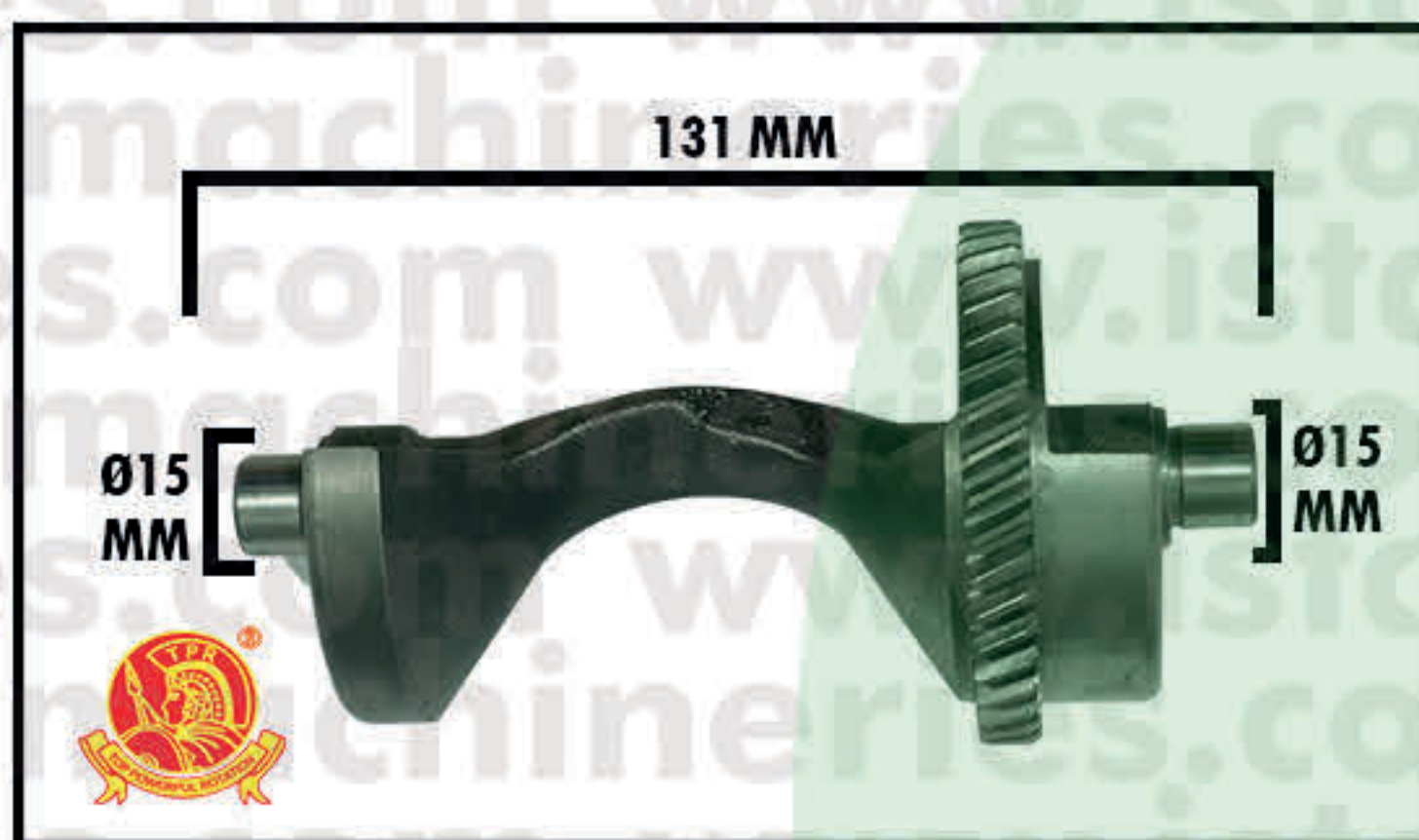
BALANCER SHAFT GX420
