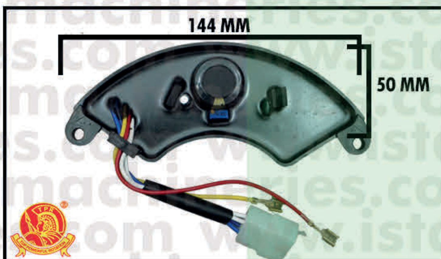
AVR PLASTIK-SABIT GFH6500
