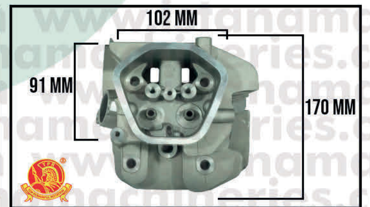
CYL HEAD ONLY GX420
