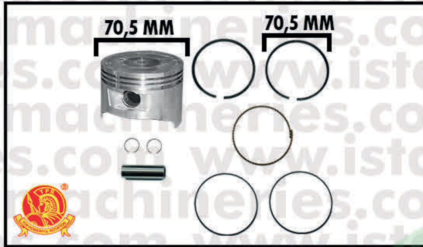
PISTON ASSY 0.50 GX220
