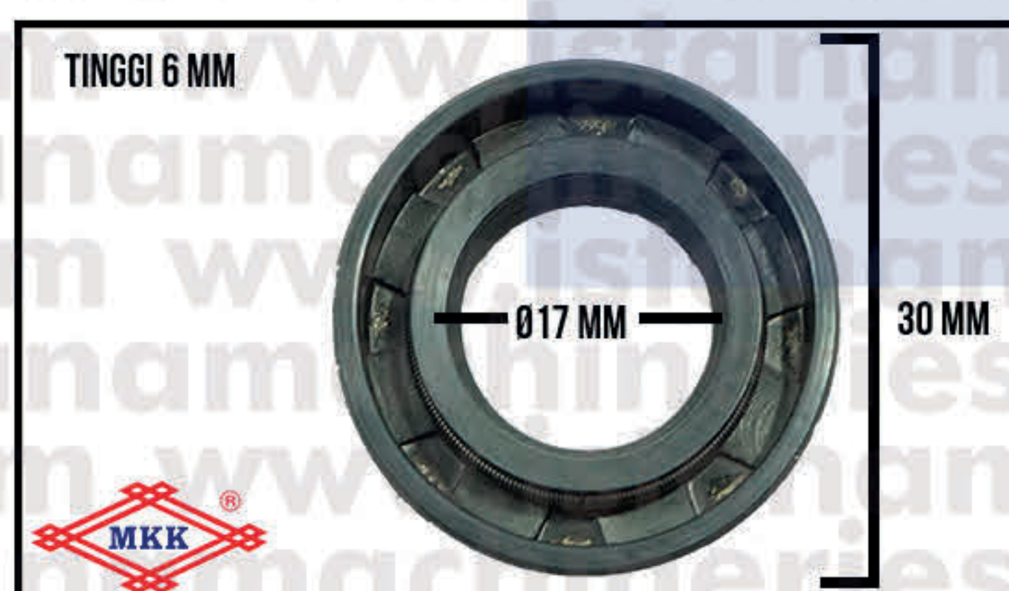
OIL SEAL CRANKSHAFT 17*30*6 M152/ET1500
