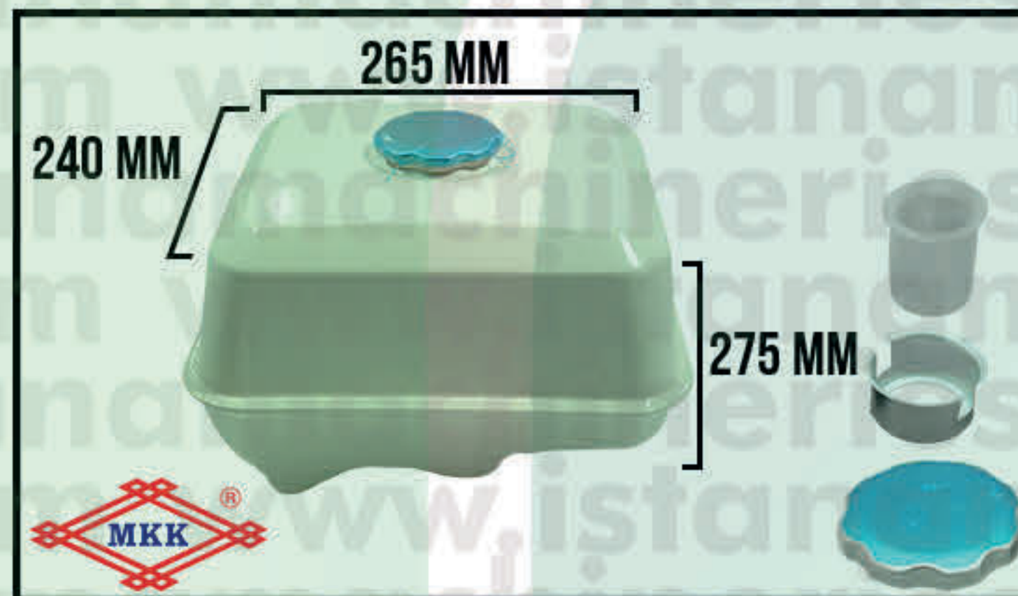
FUEL TANK ASSY "PUTIH" GX390>420
