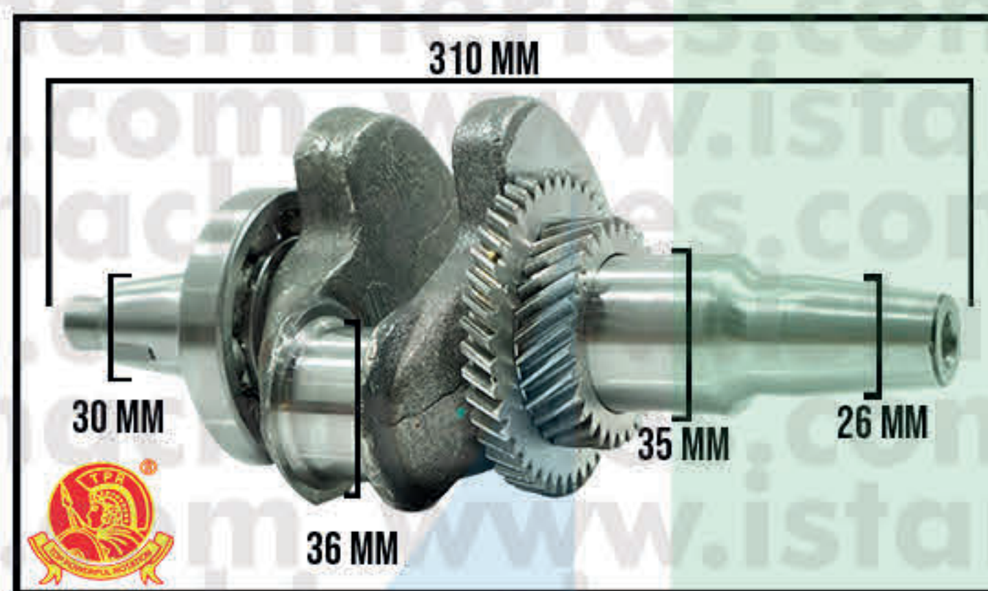
CRANKSHAFT SPIE "FOR GENERATOR" GX390/460
