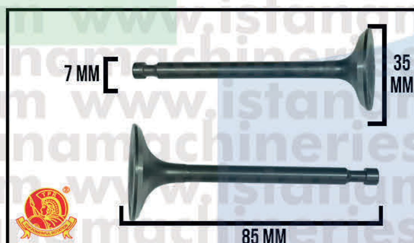
VALVE IN+EX "OLD" GX420>460
