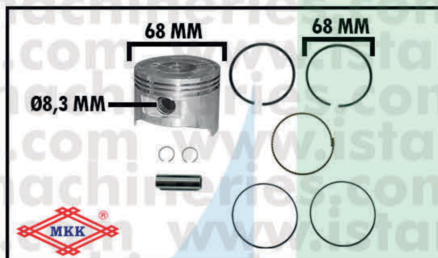
PISTON ASSY STD GX160
