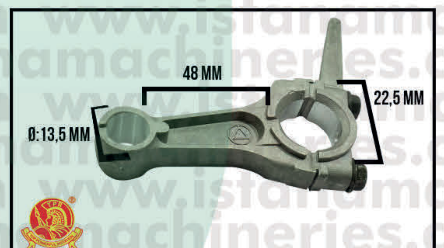
CONROD ET1500
