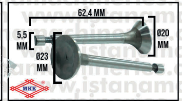
VALVE IN/EX ET1500
