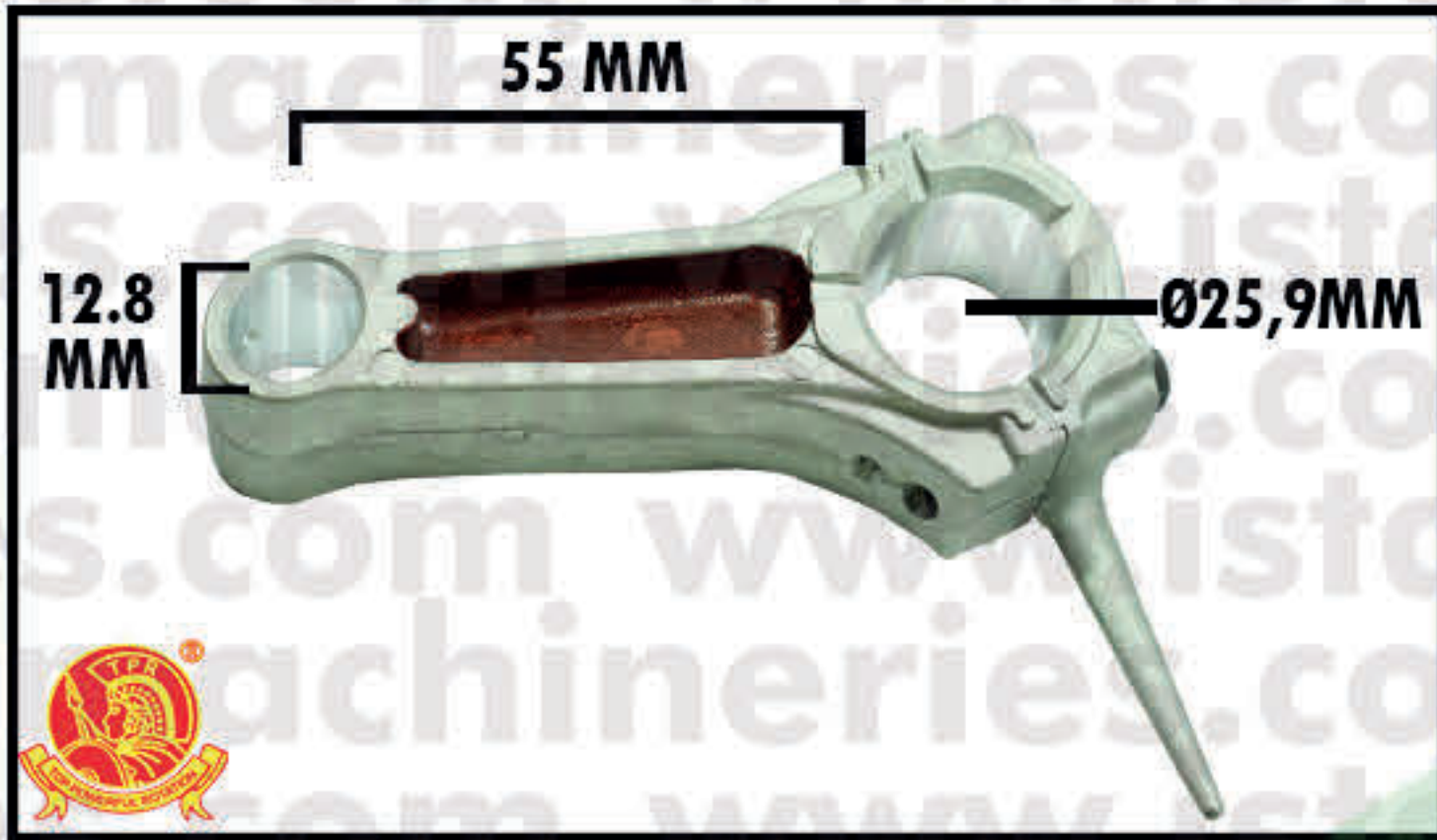
CONROD STD GX110/120
