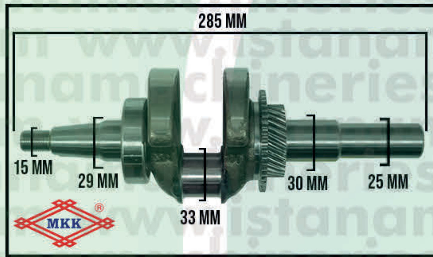
CRANKSHAFT GX270
