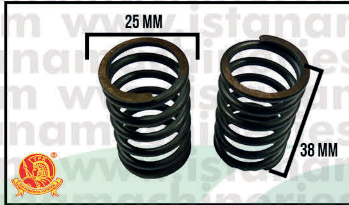
SPRING VALVE GX390>420
