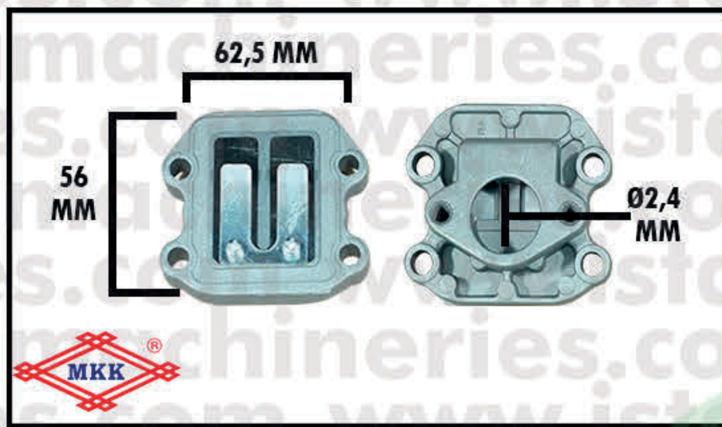
AIR BREATHER ASSY ET950
