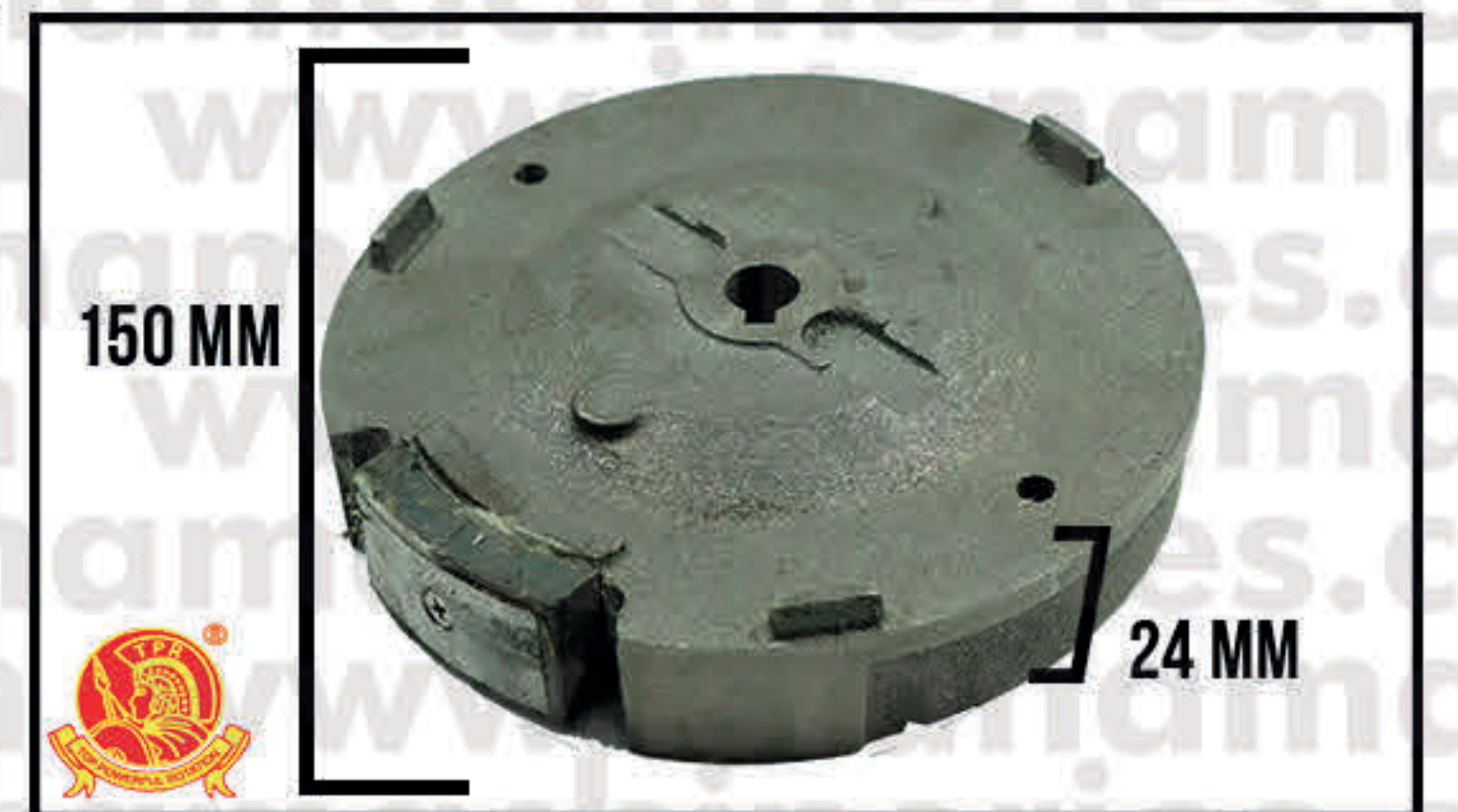
FLYWHEEL 1500
