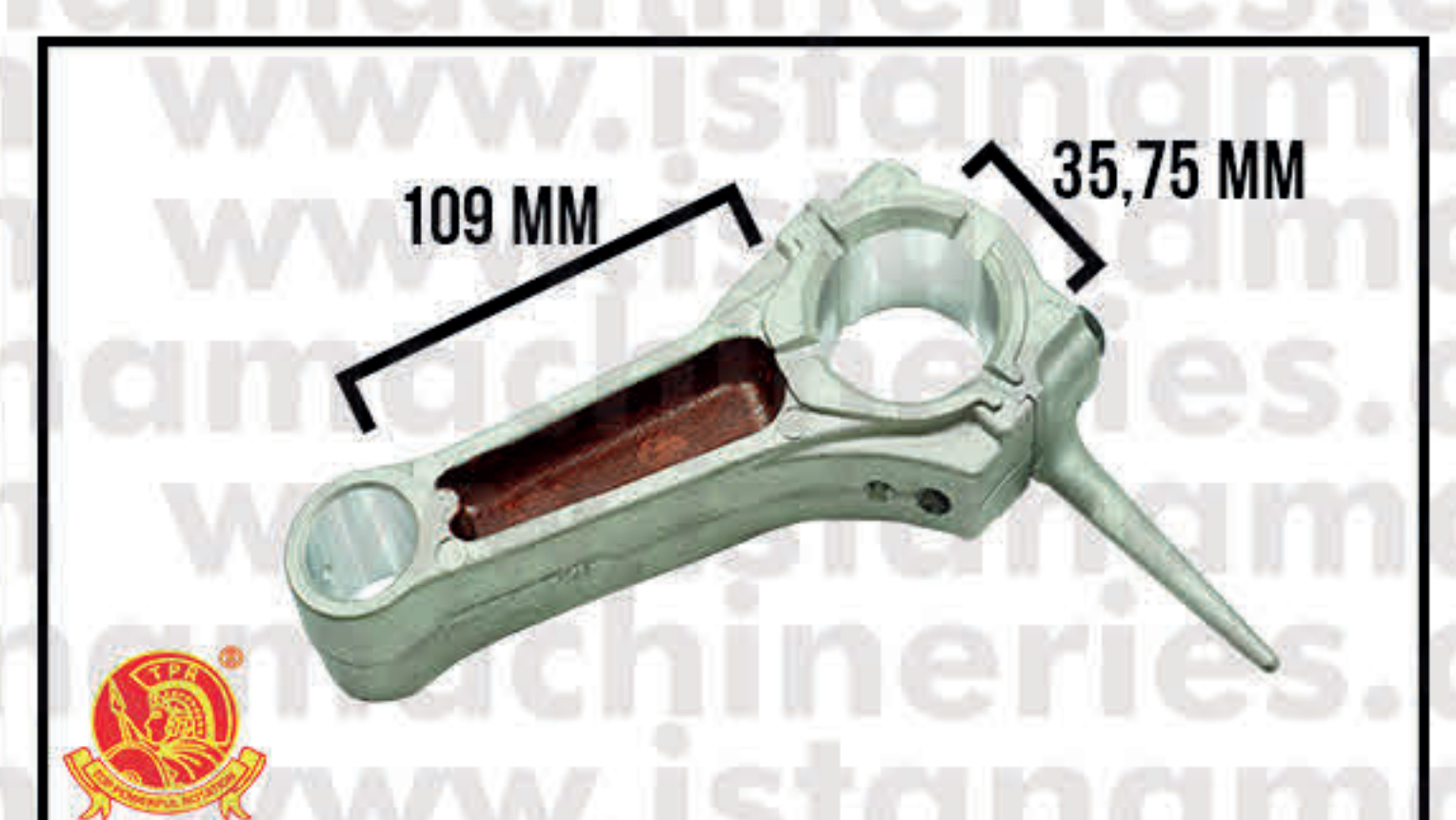
CONROD 0.25 GX340>420
