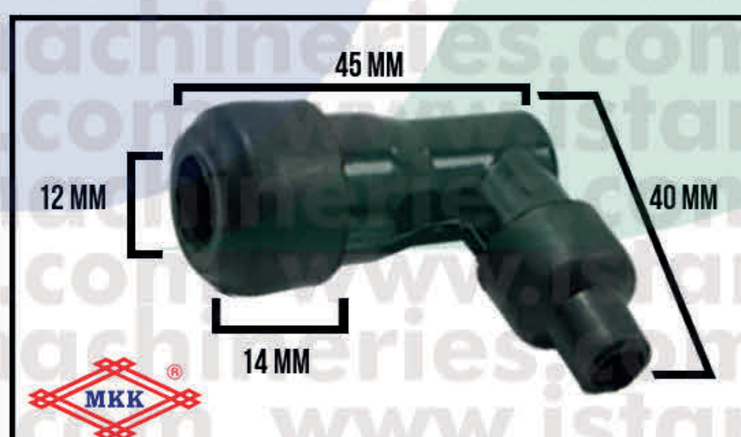
COP BUSI SHORT ET1500
