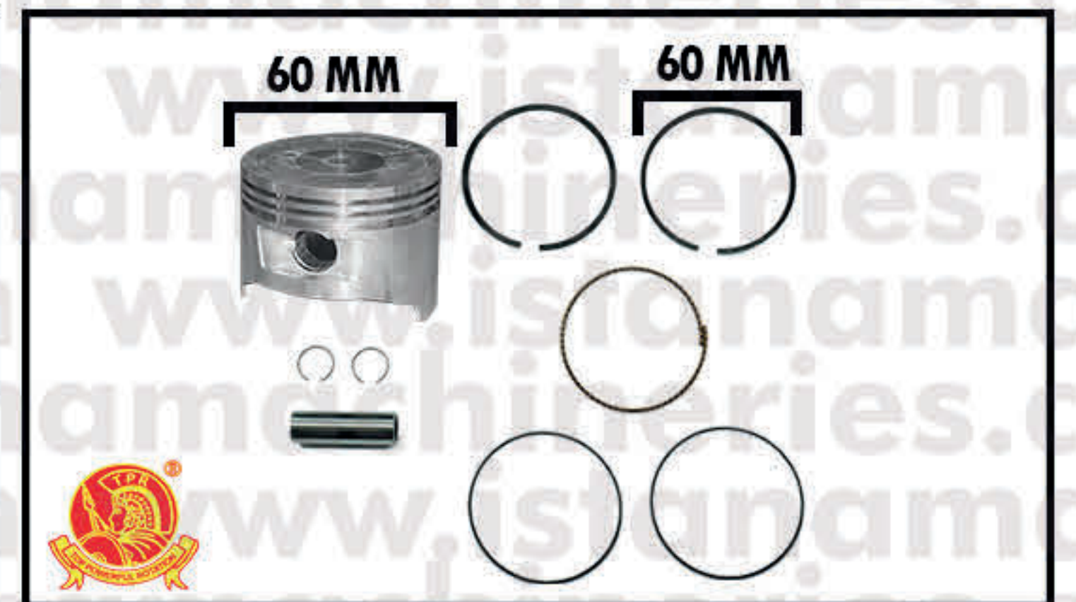
PISTON ASSY STD GX120
