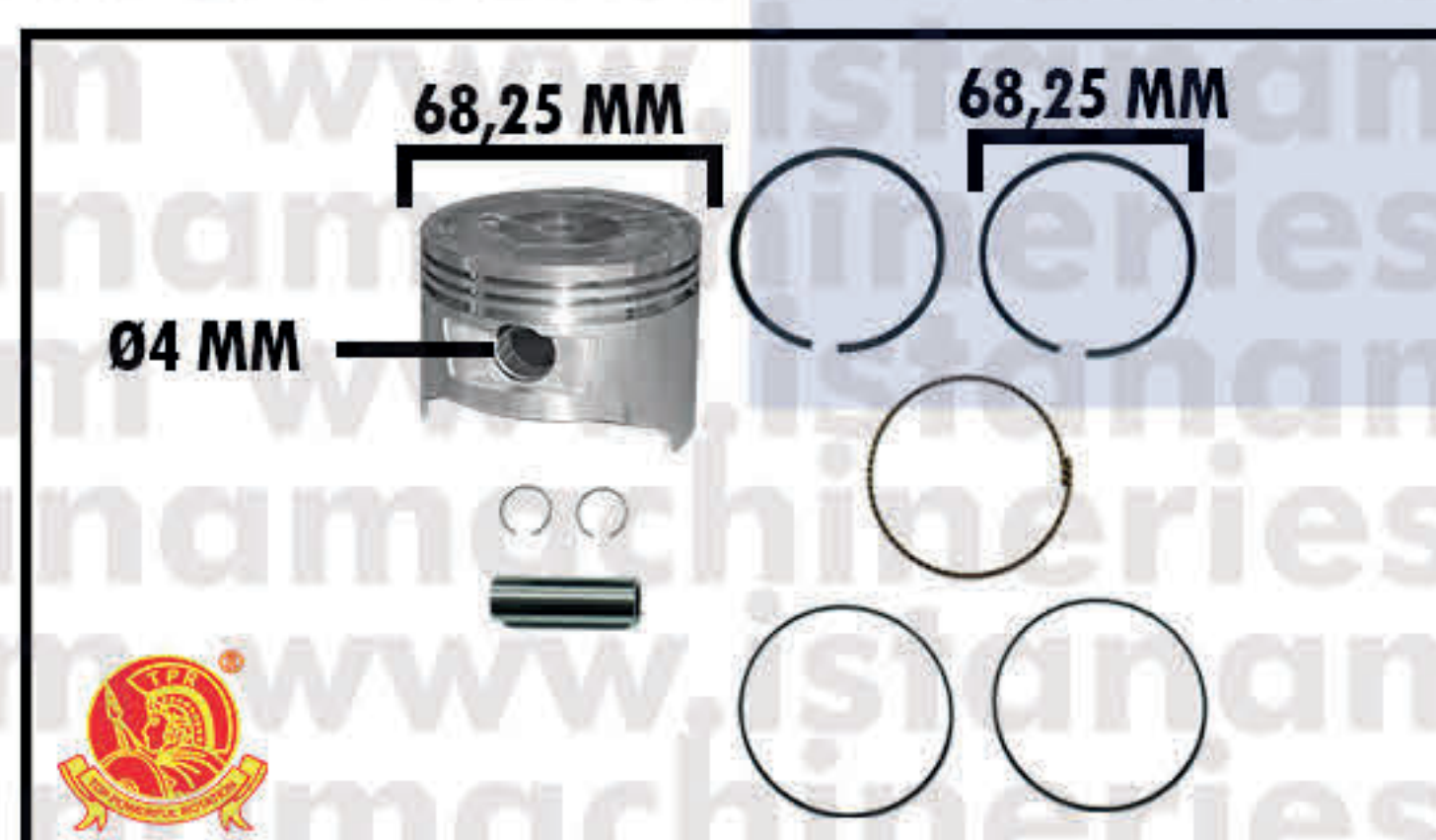
PISTON ASSY 0.25 GX200
