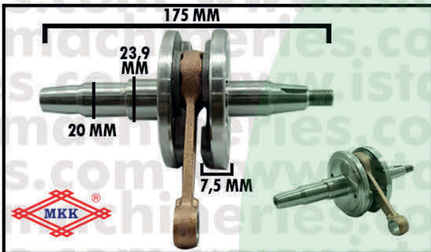
CRANKSHAFT ET950
