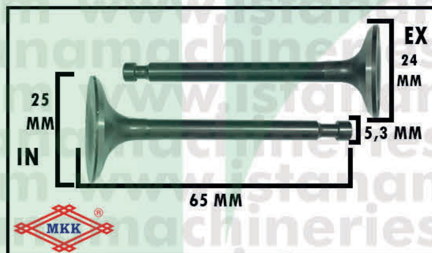
VALVE IN+EX GX 160/200
