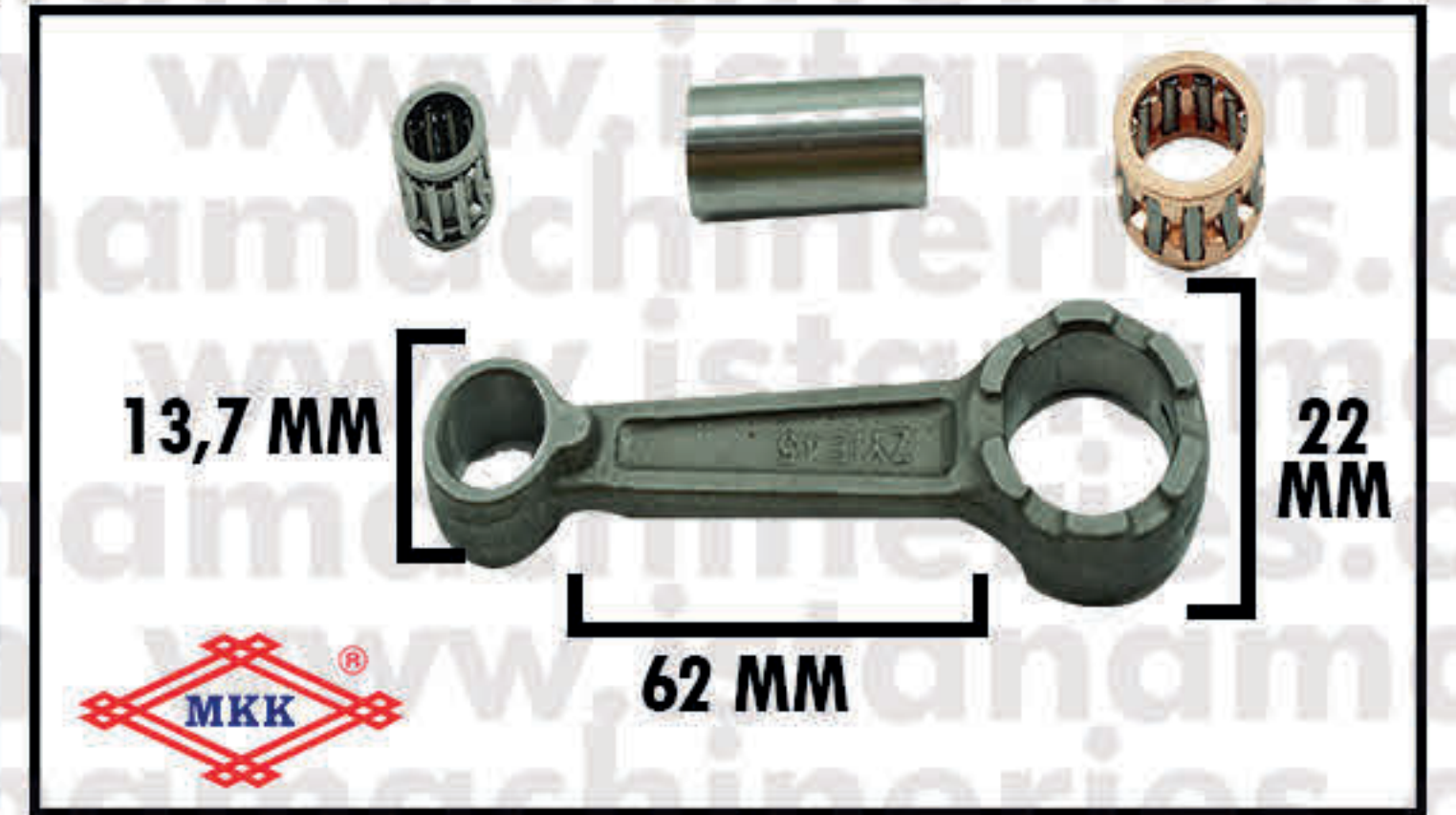
CONROD ASSY ET950
