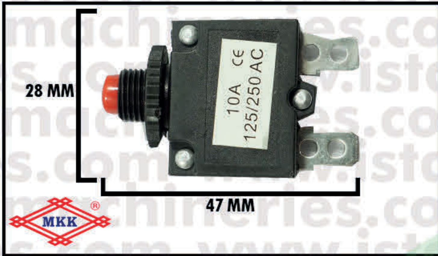
OVERLOAD PROTECTOR "5/10A" ET950
