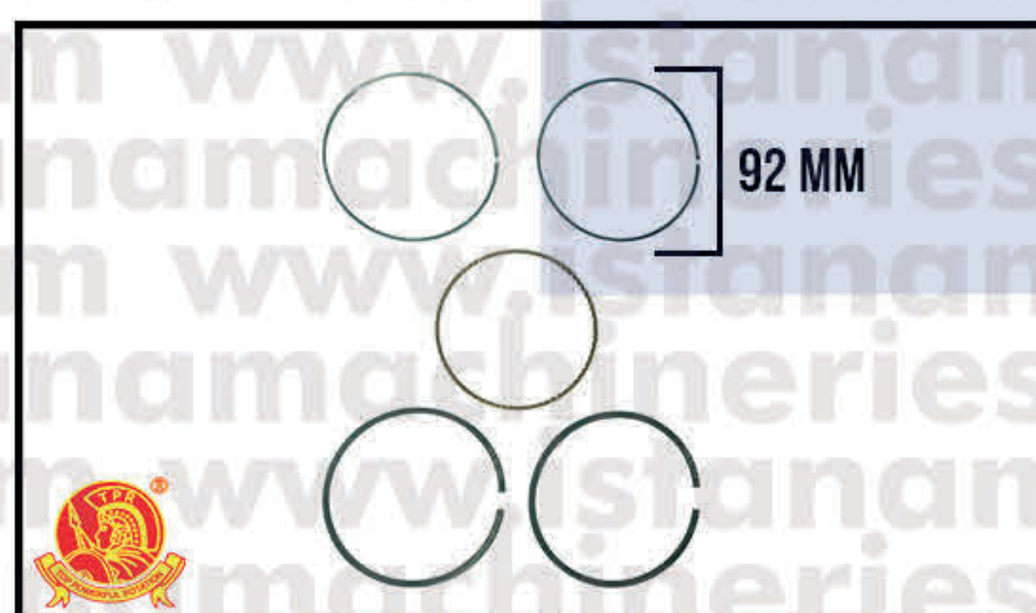
RING SET STD GX460
