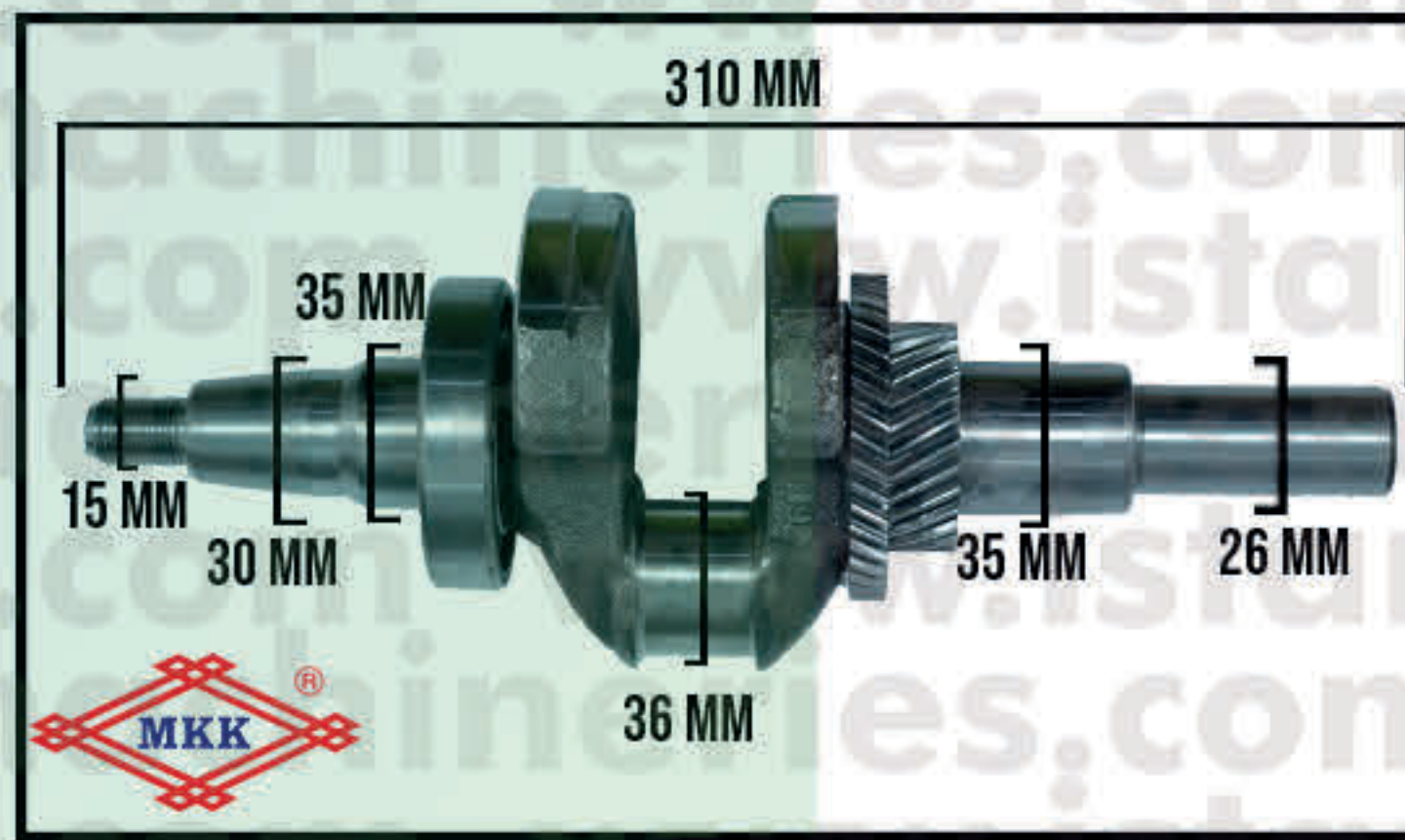
CRANKSHAFT GENERATOR GX390/420
