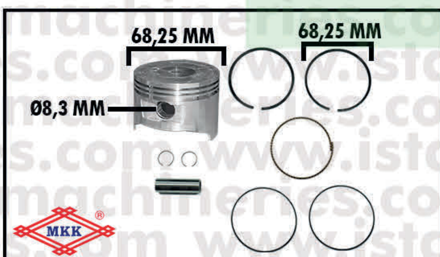
PISTON ASSY 0.25 GX160
