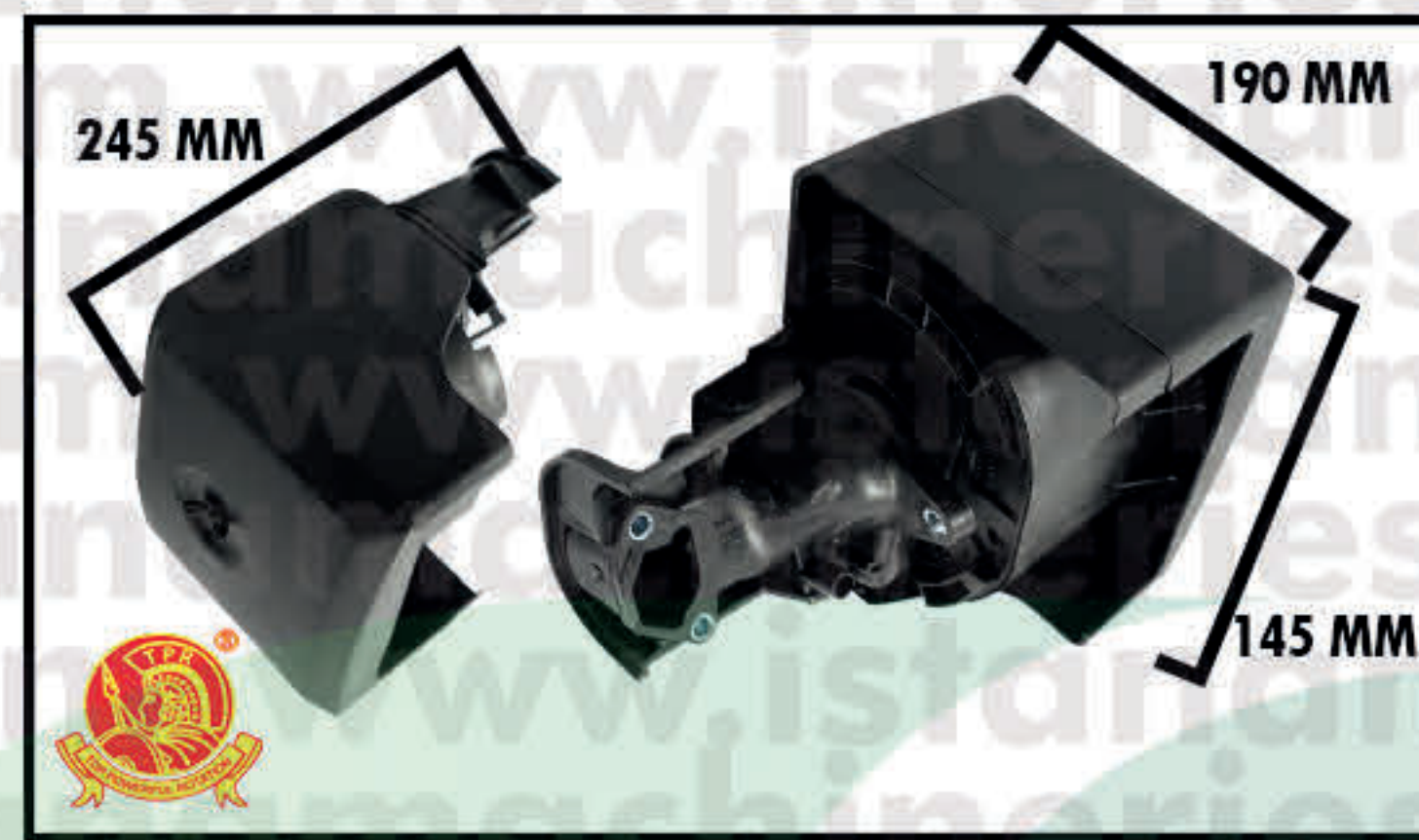
AIR CLEANER GX340-420
