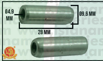
VALVE GUIDE ET1500
