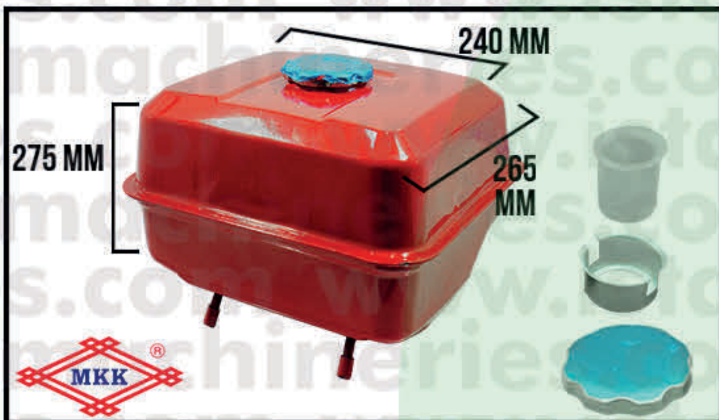
FUEL TANK ASSY "MERAH" GX390>420
