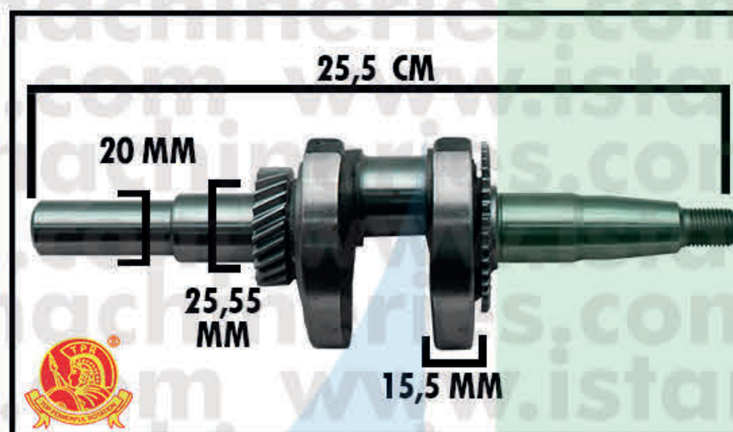
CRANKSHAFT "DRAT-SPIE" 20MM GX- 200/220
