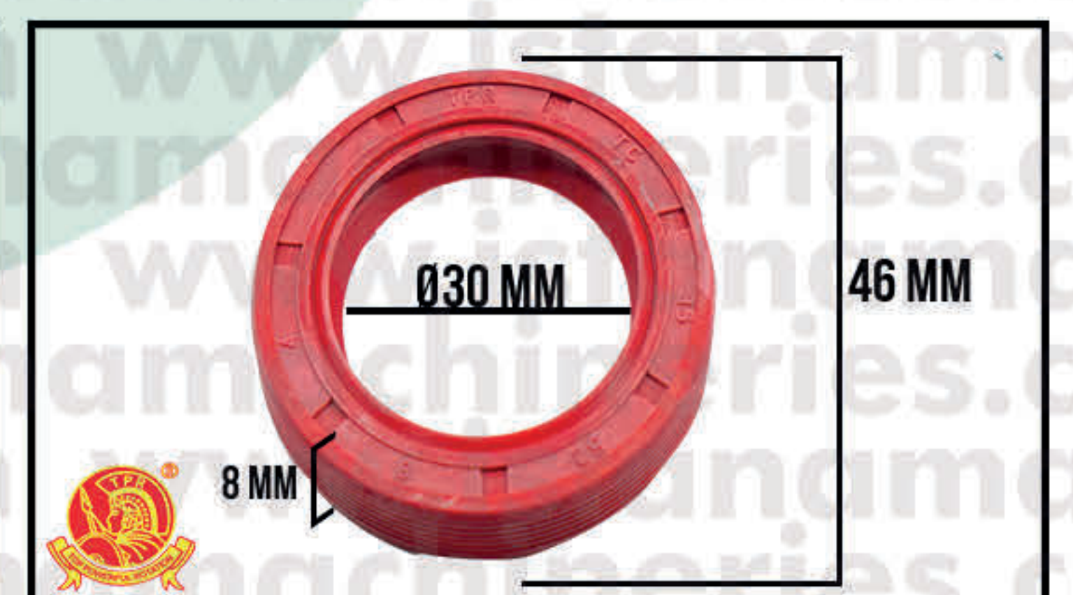
OIL SEAL CRANKSHAFT 30*46*8 GX270
