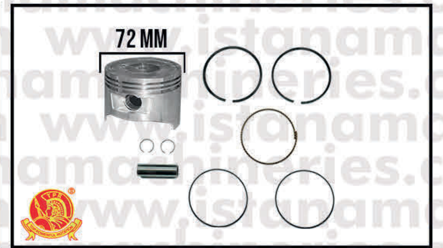
PISTON ASSY STD GX270
