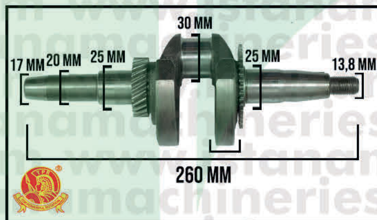
CRANKSHAFT ET4000
