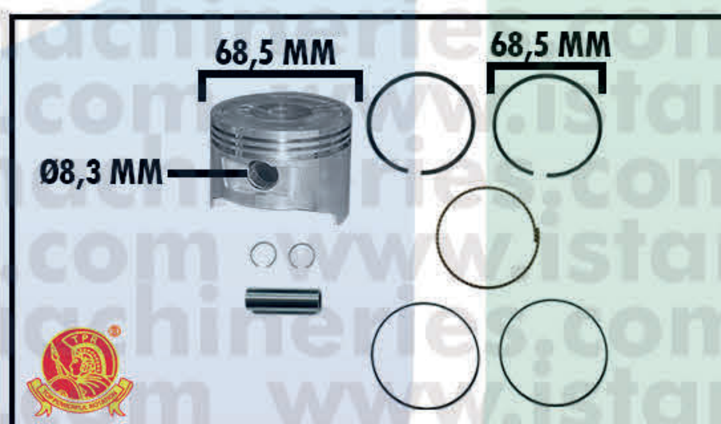
PISTON ASSY 0.50 GX160
