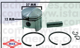
PISTON ASSY 37MM BG-328
