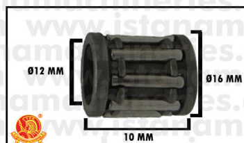
BEARING PIN PISTON BG318/328
