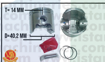
PISTON ASSY CG411
