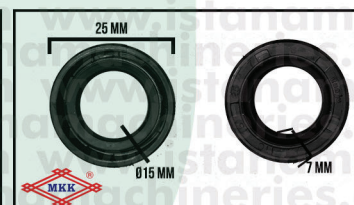
OIL SEAL 15-25-7 BG221>328
