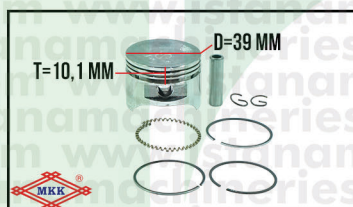
PISTON ASSY "ECO" 40MM MX-35
