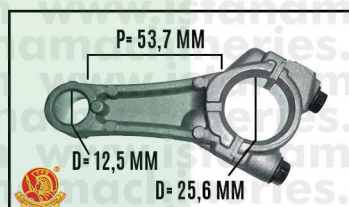
CONROD SM4605/PM5103
