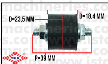
ENGINE MOUNTING MX-35
