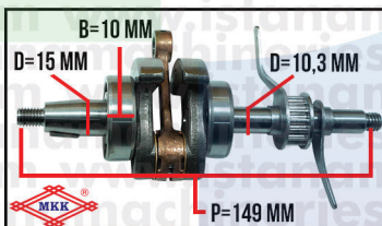
CRANKSHAFT MX-35
