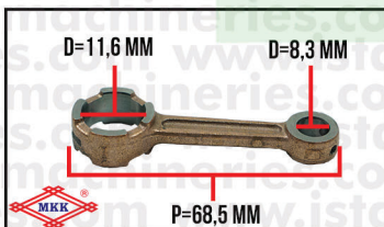
CONROD ONLY MX-35
