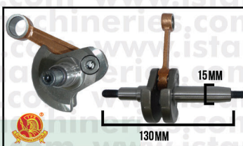
CRANKSHAFT BG-328
