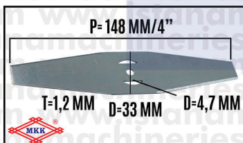
PISAU POTONG 4 INCH MB-12
