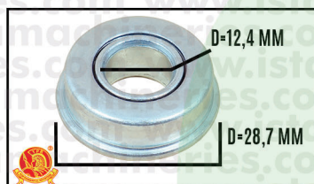
BEARING FOR WHEELS PM5103
