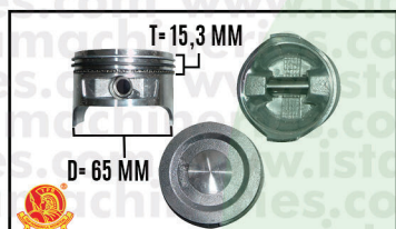
PISTON ASSY SM4605/PM5103
