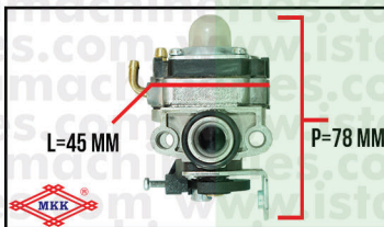
CARBURATOR ASSY MX-35
