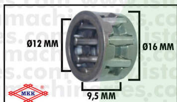
BEARING PIN CRANK BG-328
