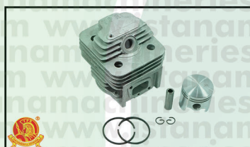
CYLINDER BLOCK ASSY CG430
