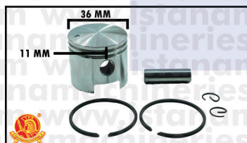
PISTON ASSY 36MM BG-318
